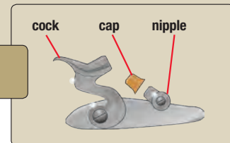
Parts of the Percussion Lock
